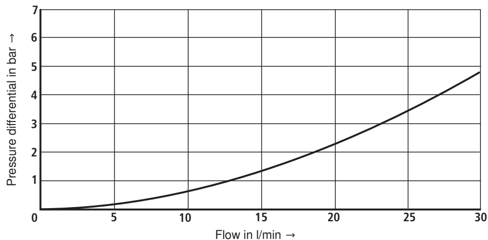
Pressure differential P1 → P2
